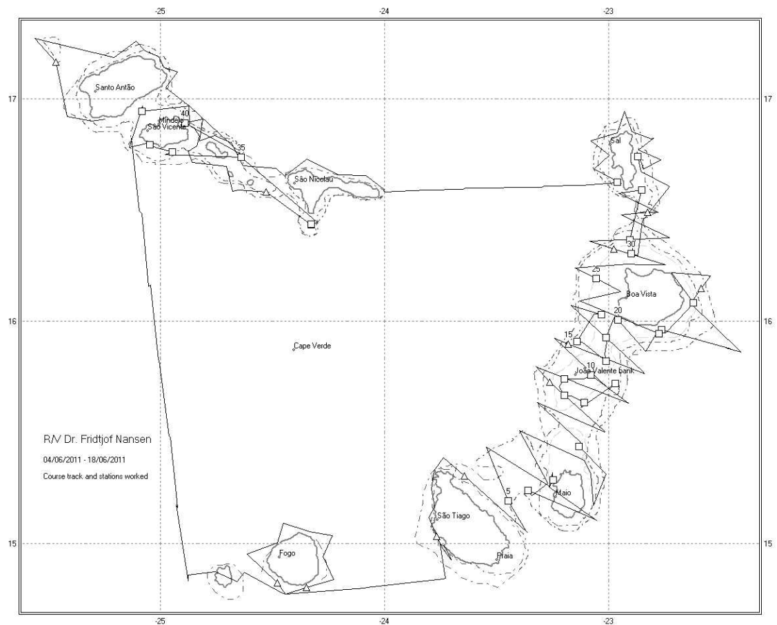
Figure 1.1. Course track with bottom trawl (□) and pelagic (Δ) trawl stations. The 100, 500 and 1000 m depth contours are indicated.
