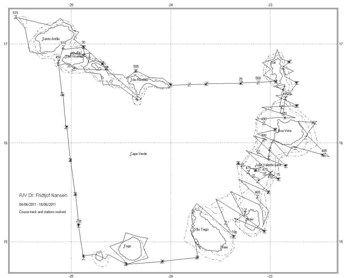
Figure 1.2. Course track with hydrographic (Z), plankton (X) and benthos (◇) stations. The 100, 500 and 1000 m depth contours are indicated.
