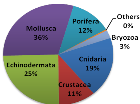
Figure 3.10. Global composition in number (left) and weight (right) by main Phylum of the epibenthic fauna collected during Cape Verde Survey.
