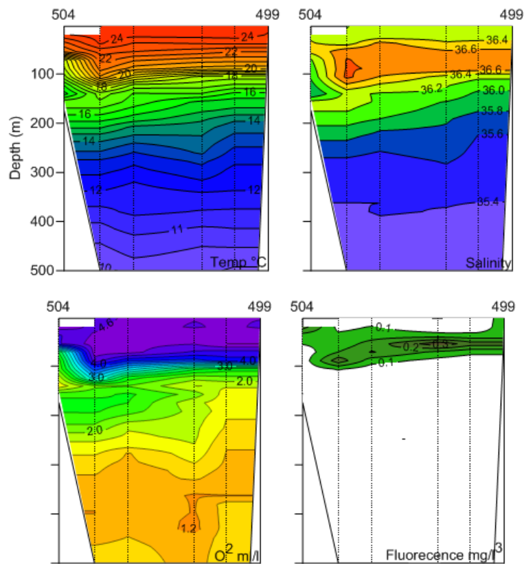
Figure 3.7. Temperature, salinity, dissolved oxygen and fluorescence observed on the transect between Sal and São Nicolau.
