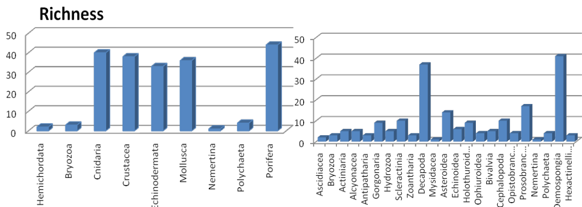
Figure 3.12. Richness (morphospecies number) by Phylum (left) and Class (right).
