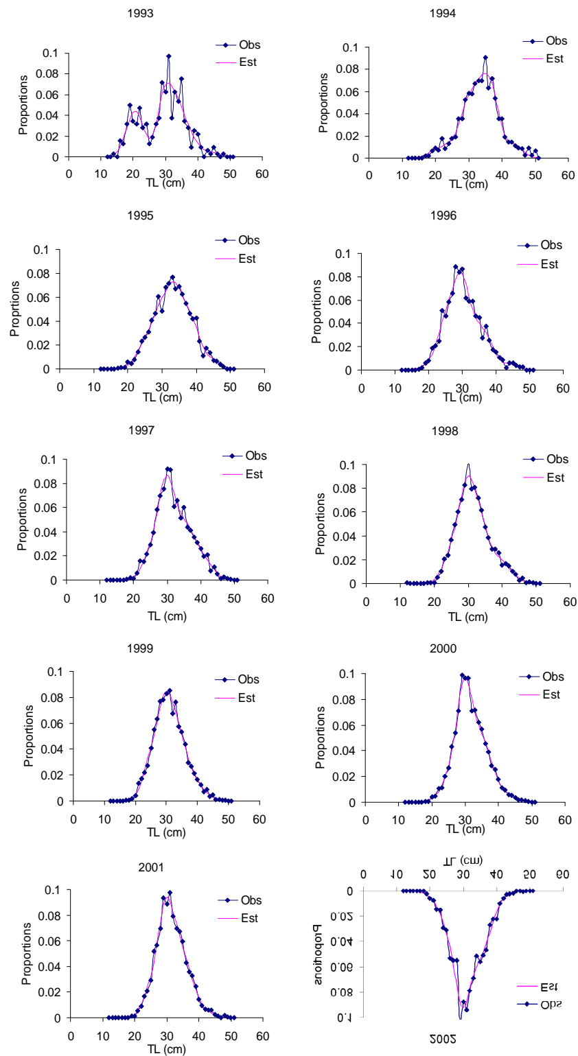
Figure 3.6.: Observed and estimated length-frequencies for C. taeniops , 1993-2002
