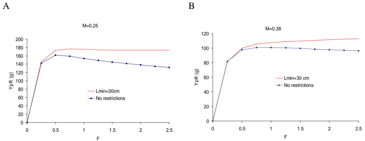
Figure 3.10.: Estimated YpR for two M -values scenarios setting the minimum size of capture at 30 cm ( L_{min}=30 cm) and without restrictions in the size of capture
