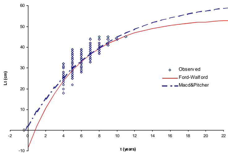
Figure 3.5.: Growth curves obtained from aged sub-sample(Ford-Walford), fitted through minimisation and from Macdonald and Pitcher re-estimation. (Macd&Pitcher).
