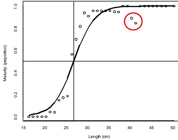
Figure 3.3.: Maturity at length ogive for C. taeniops , 1993-2002.
