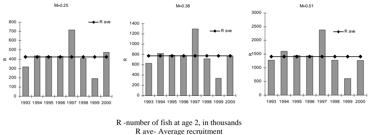
Figure 3.8: Estimated recruitment R and the average recruitment for C. taeniops in 1993-2000 period, giving three different scenarios of M -values.
