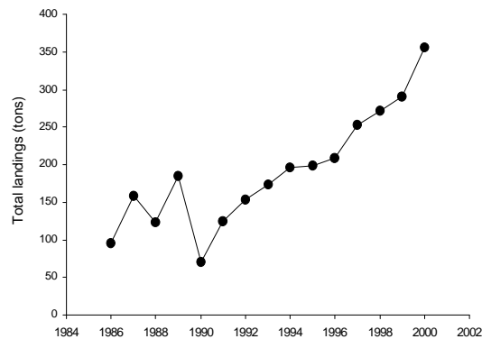
Figure 1.2.: A) Cephalopholis taeniops (Valenciennes, 1828). B) C. taeniops total artisanal landings from 1986 to 2000, Cape Verde archipelago.
