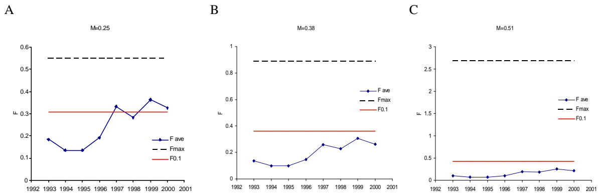
Figure 4.1.: Comparison of the F_{0.1} and F_{max} resulted from YpR analysis with the \bar{F} resulted from VPA for the different M scenarios.
